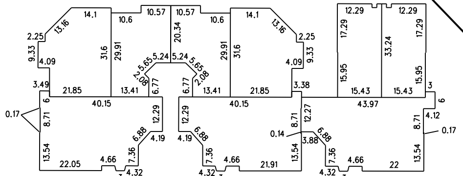
BUILDING "A" TYPE (TYPICAL) NOT TO SCALE
