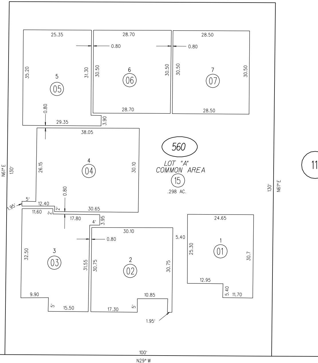
FIRST LEVEL
