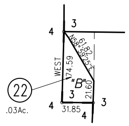
DETAIL "A" 1"=100'
