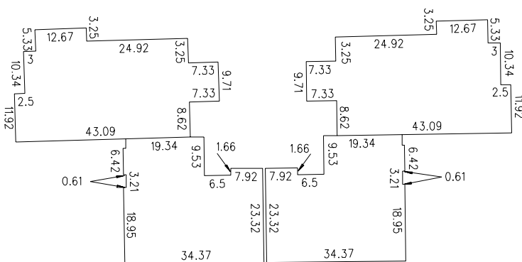
BUILDING "A" TYPE (TYPICAL) NOT TO SCALE
