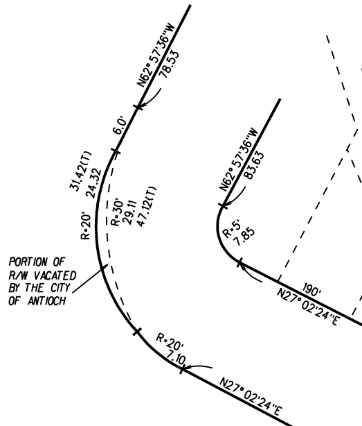
DETAIL OF LOT "2" NORTHWEST CORNER 1"=10'
