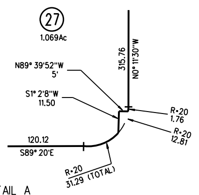
DETAIL A 1"=50'
