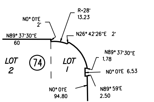
DETAIL A 1" = 50'
